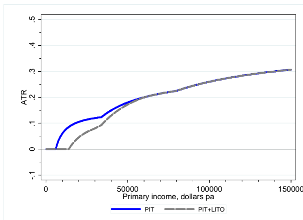
Figure 3.1a ATRs: PIT scale and LITO, 2008-09
