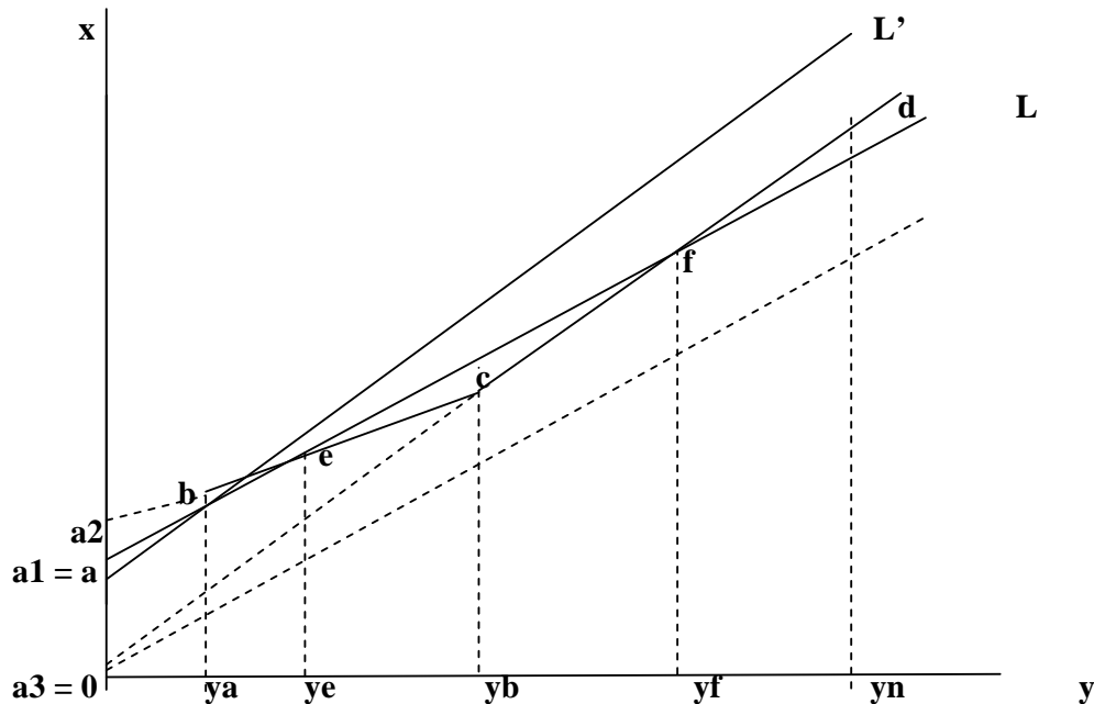
Figure A2: Non-convex piecewise linear income tax
