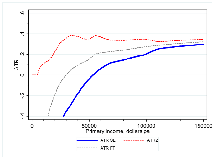
Figure 4.3b MTRs: PIT + LITO+FTBs + ML
