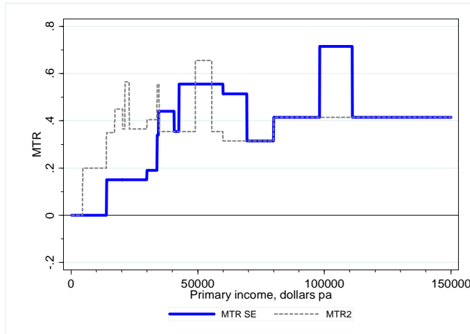
Figure 4.3a MTRs: PIT + LITO + FTBs + ML
